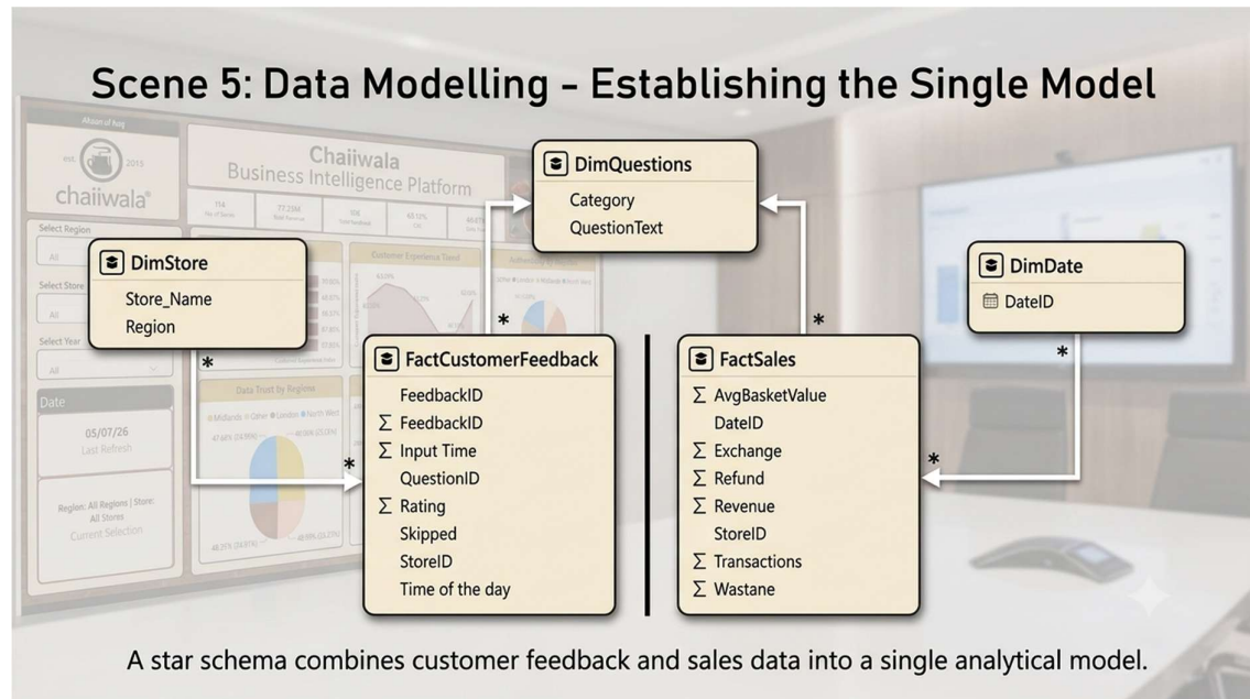
Figure 4: An illustration of a Star Schema data modelling where all customer feedback and sales data kept into a single analytical model
